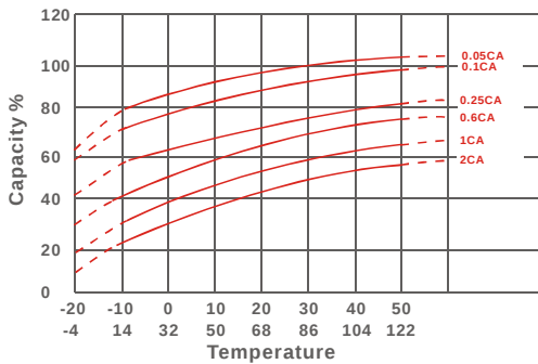
Effect of Temperature on Capacity 25 (77 °)
