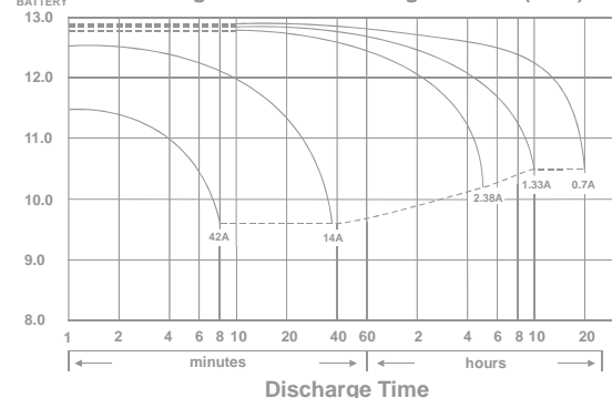
(v) FOR 12V BATTERY 13.0 Discharge Time VS. Discharge Current (25 )
